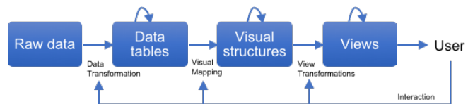
Figure 1. VRiDaM architecture.
