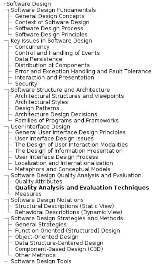
Figure 10. SWEBOK SD concepts (in bold) conveyed by Angry Nerds.
