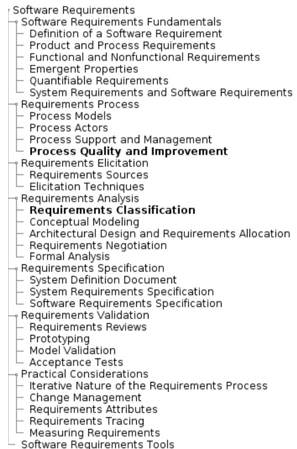
Figure 7. SWEBOK concepts (in bold) conveyed by ReqAbdeck.
