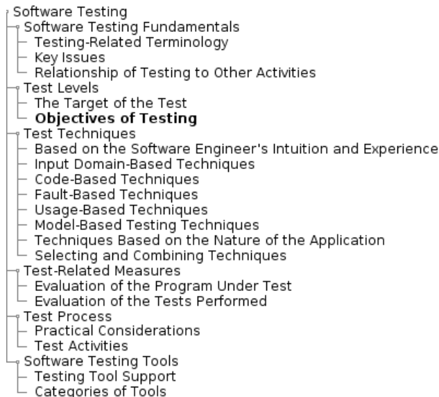
Figure 9. SWEBOK ST concepts (in bold) conveyed by Angry Nerds.
