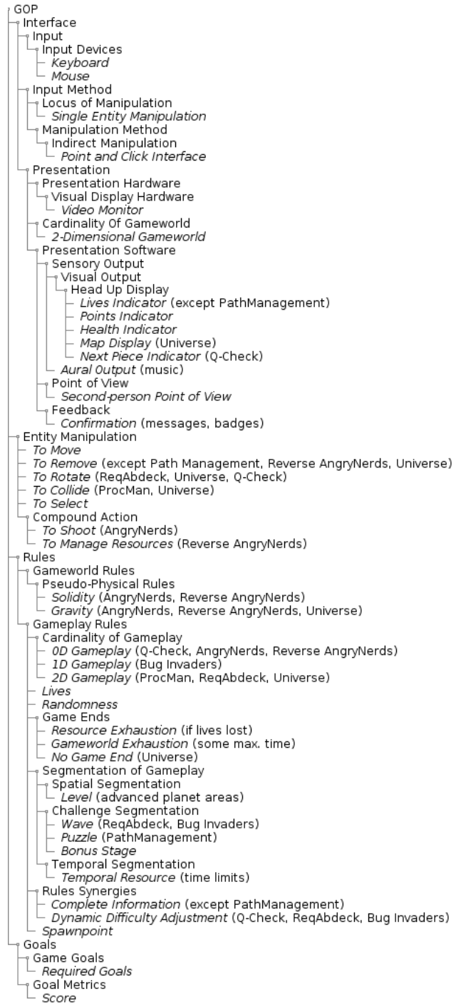
Figure 20. GOP concepts (in italics) utilized by SWE4SE.
